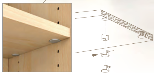
Shelf clip detail
